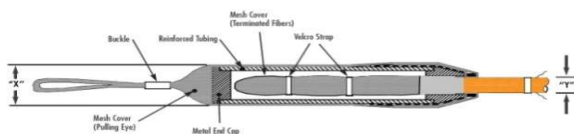
Encapsulated Protection Sleeve
